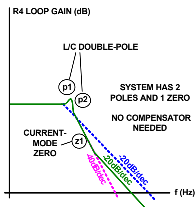
FIGURE 65. UNCOMPENSATED R4™ OPEN-LOOP RESPONSE
