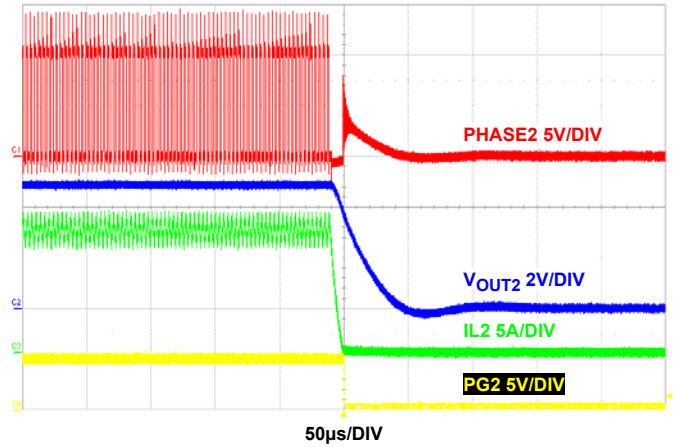
FIGURE 55. CH2 OCP
